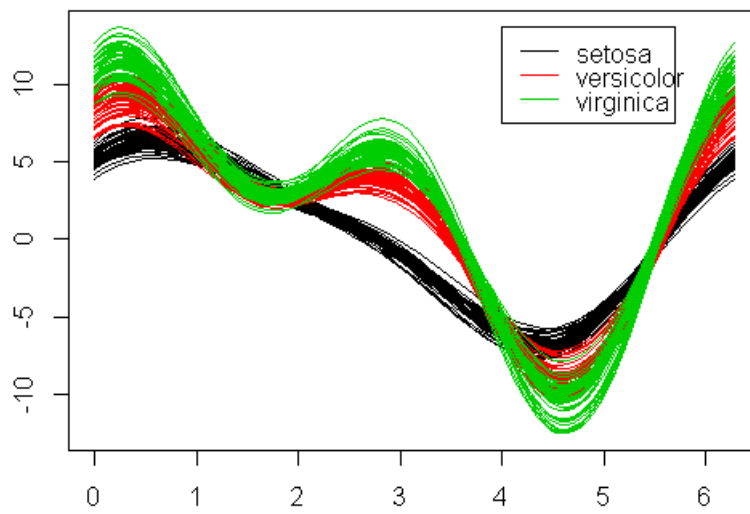
Andrews' Curves
